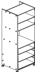
3 DRAWER OVEN TOWER 600MM
