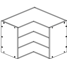
SHORT CORNER WALL CABINET 600 x 600MM
