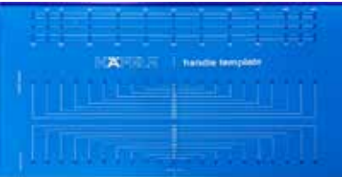
HANDLE JIG TEMPLATE 001.35.090
