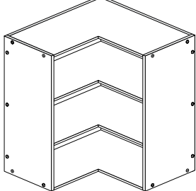
TALL CORNER WALL CABINET 600 x 600MM
